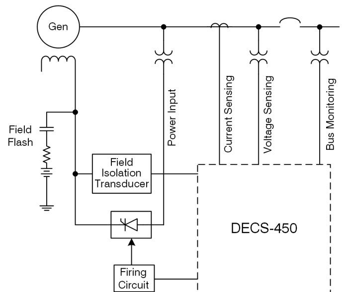
Figure 1 - DECS-450 Connection Diagram for a Typical Application
