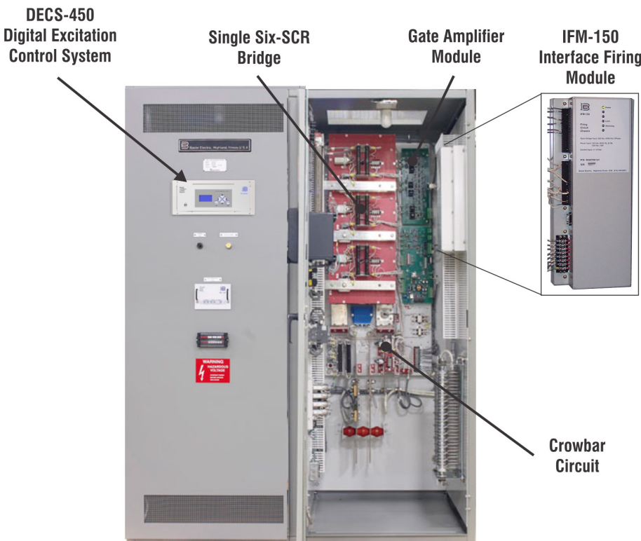
Figure 2 - Typical DECS-450 with Single Rectifier Bridge
